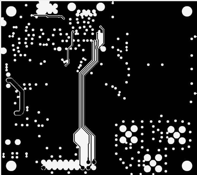
P026922 Innerlayer 3 Image (topview)
