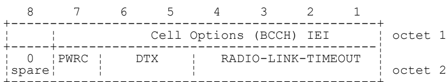
FIGURE 10.17/3GPP TS 04.08 Cell Options (BCCH) information element
