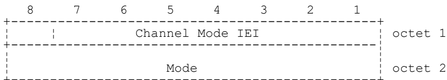
FIGURE 10.20/3GPP TS 04.08 Channel Mode information element
