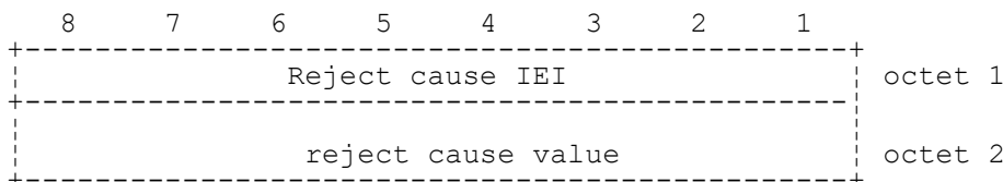
FIGURE 10.66/3GPP TS 04.08 Reject Cause information element
