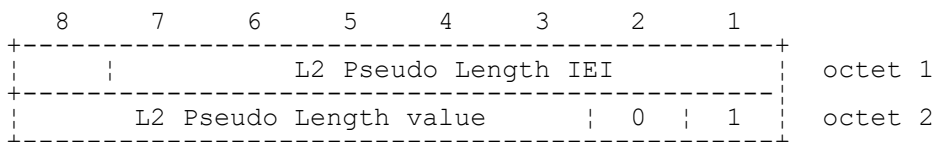
FIGURE 10.37/3GPP TS 04.08 L2 Pseudo Length information element
