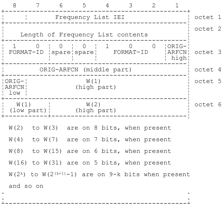
FIGURE 10.29/3GPP TS 04.08 Frequency List information element (Range 512 format)
