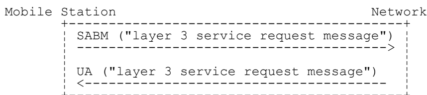
Figure 3.1/3GPP TS 04.08 Service request and contention resolution
