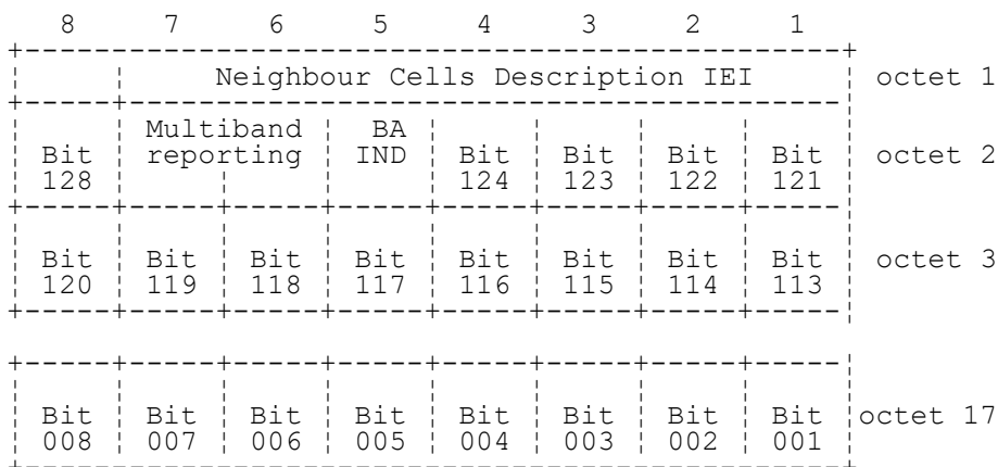
FIGURE 10.40a/3GPP TS 04.08 Neighbour Cells Description 2 information element
