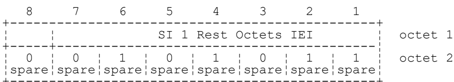
FIGURE 10.50/3GPP TS 04.08 SI 1 Rest Octets information element
