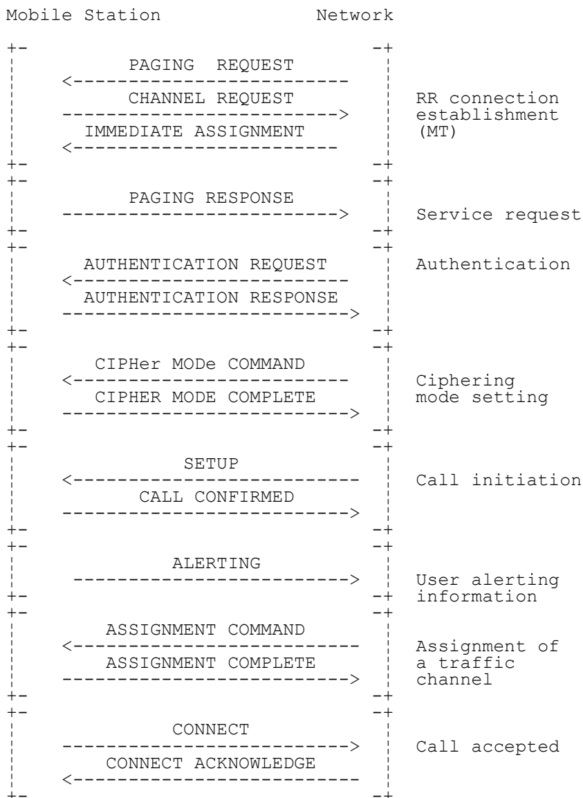
Figure 7.11b/3GPP TS 04.08 - Mobile terminating call establishment with OACSU (late assignment)
