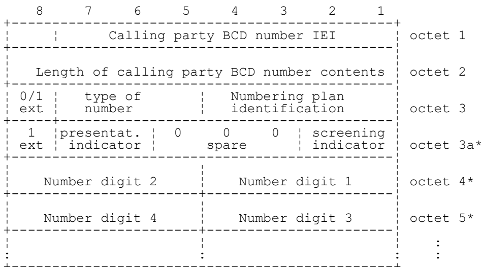
FIGURE 10.75/3GPP TS 04.08 Calling party BCD number information element
