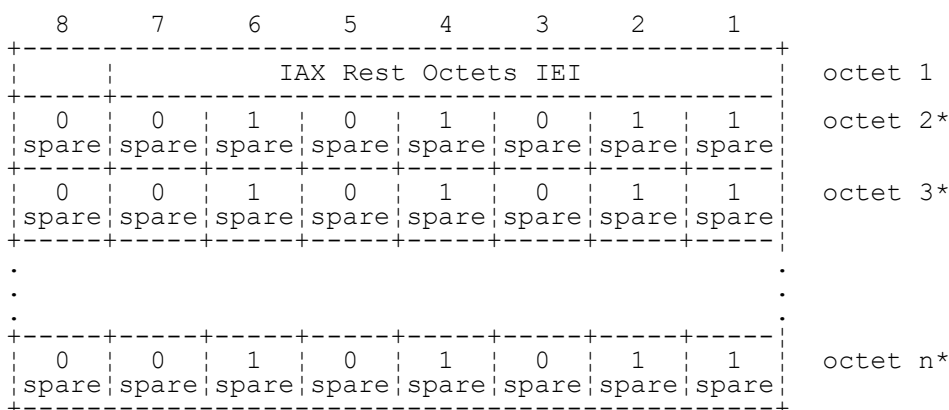
FIGURE 10.36/3GPP TS 04.08 IAX Rest Octets information element
