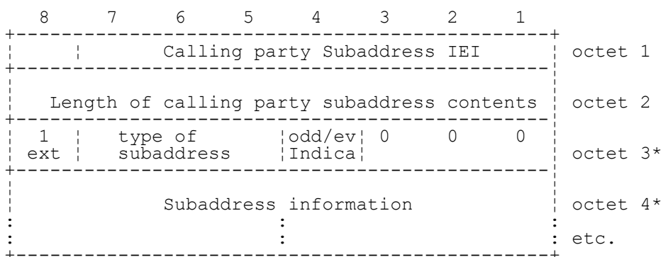
FIGURE 10.76/3GPP TS 04.08 Calling party subaddress
