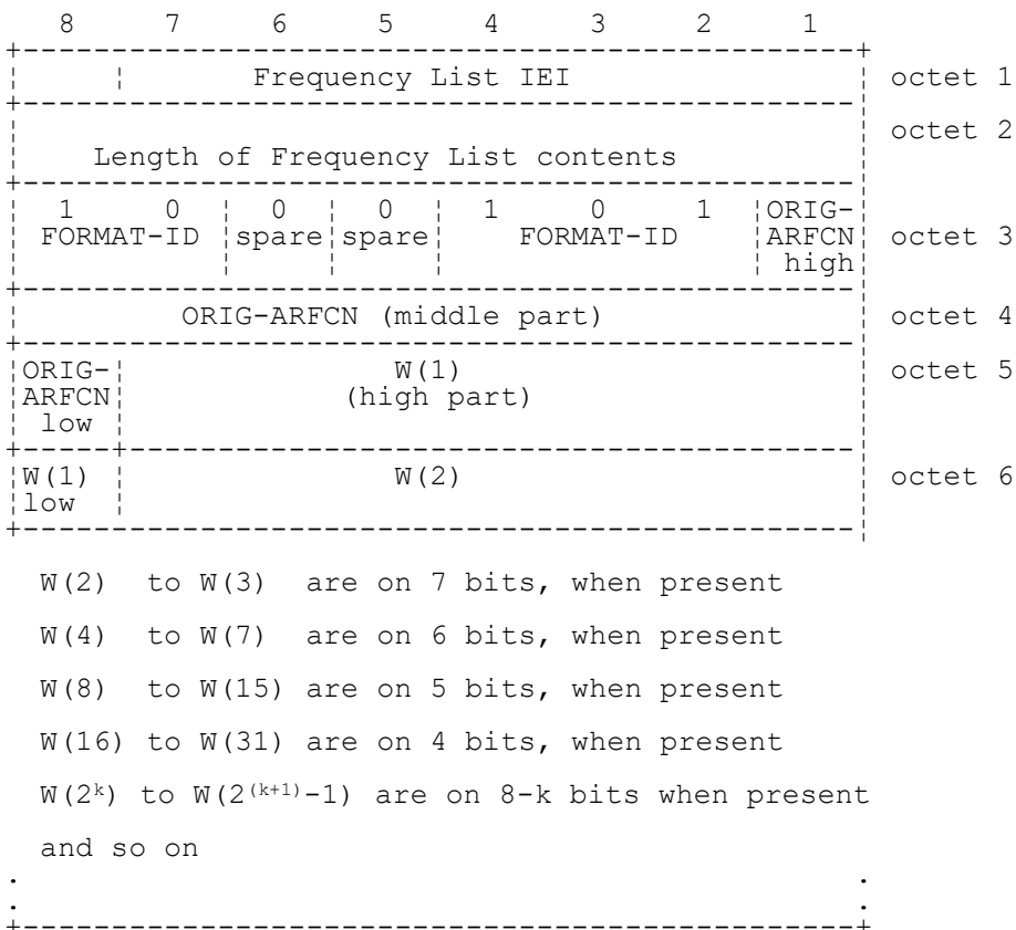
FIGURE 10.30/3GPP TS 04.08 Frequency List information element (Range 256 format)
