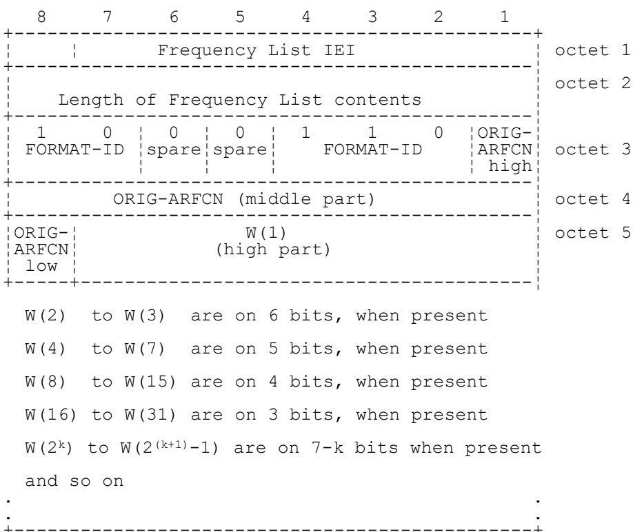
FIGURE 10.31/3GPP TS 04.08 Frequency List information element (Range 128 format)
