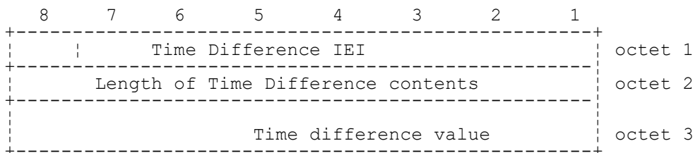
FIGURE 10.58/3GPP TS 04.08 Time Difference information element
