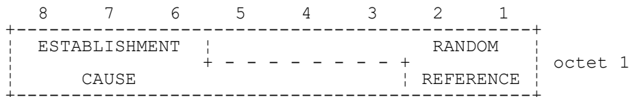
FIGURE 9.1/3GPP TS 04.08 CHANNEL REQUEST message content
