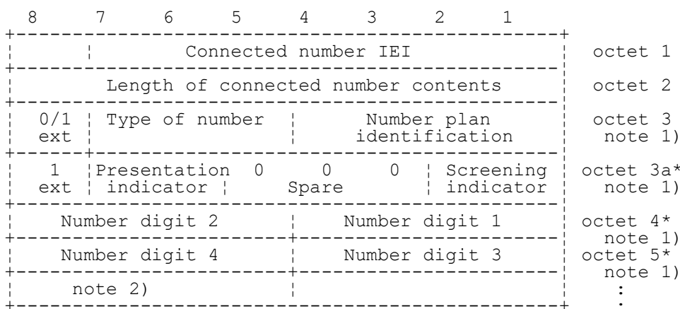
Figure 10.80/3GPP TS 04.08
