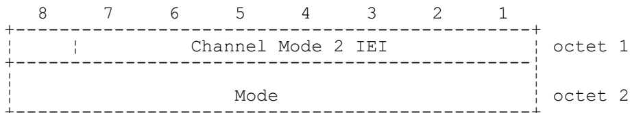
FIGURE 10.21/3GPP TS 04.08 Channel Mode 2 information element
