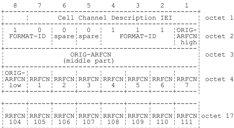
FIGURE 10.15/3GPP TS 04.08 Cell Channel Description information element, variable bit map format
