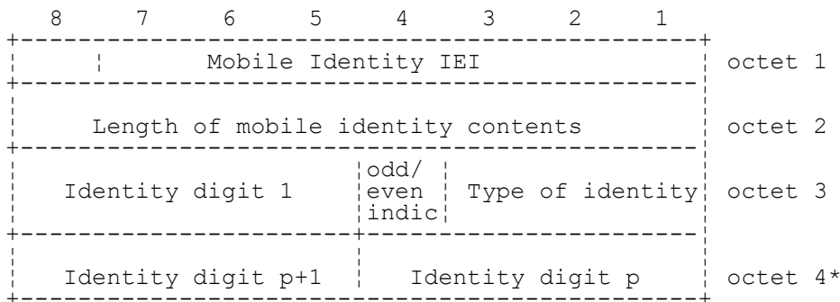
FIGURE 10.5/3GPP TS 04.08 Mobile Identity information element
