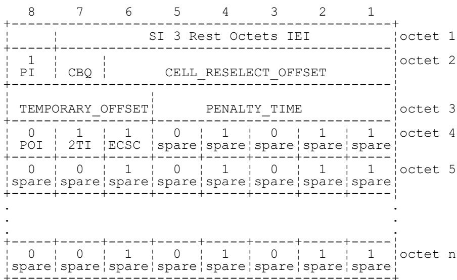
FIGURE 10.52i/3GPP TS 04.08 SI 3 Rest Octets information element for PI=H & POI=L & 2TI=H & ECSC=L
