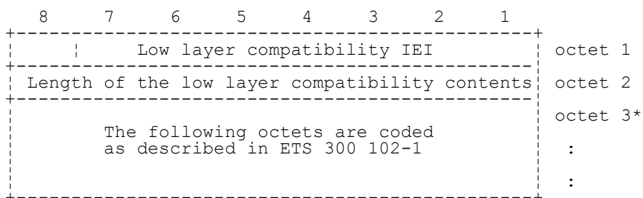
FIGURE 10.85/3GPP TS 04.08 Low layer compatibility information element
