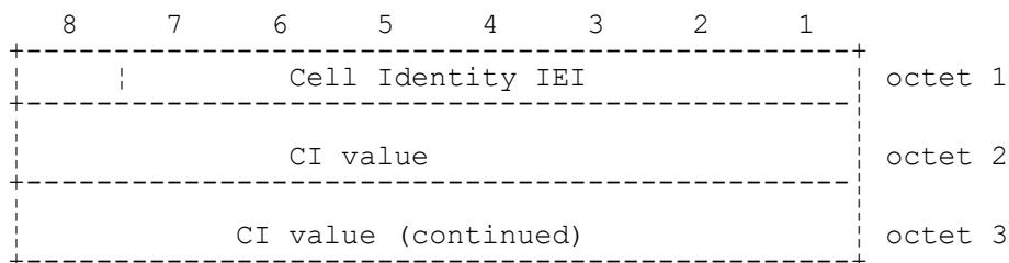
FIGURE 10.2/3GPP TS 04.08 Cell Identity information element
