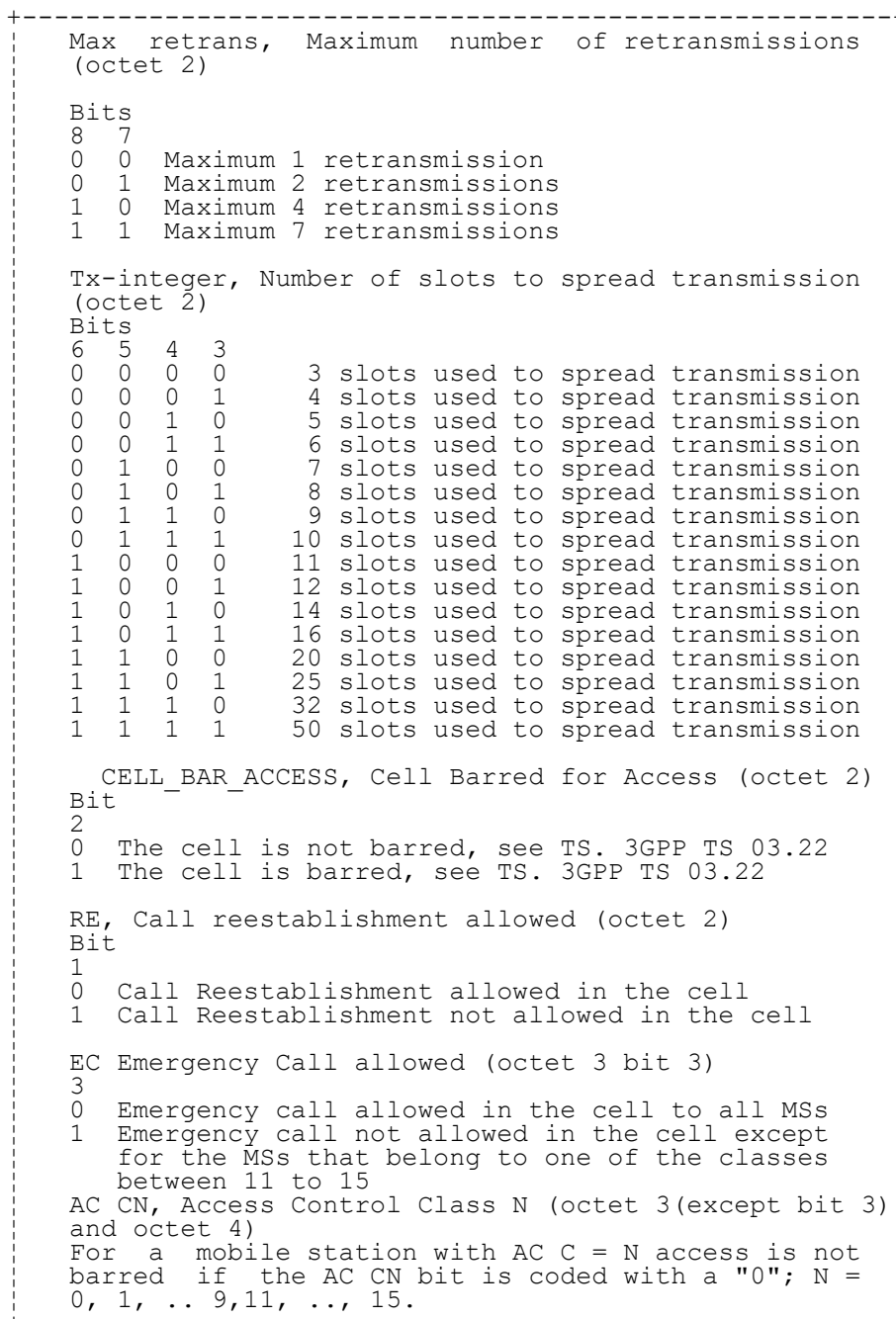
FIGURE 10.47/3GPP TS 04.08 RACH Control Parameters information element
