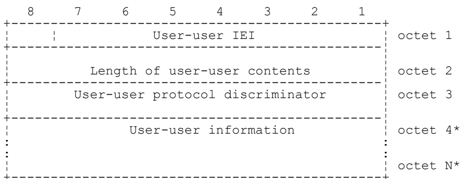
FIGURE 10.92/3GPP TS 04.08 User-user information element
