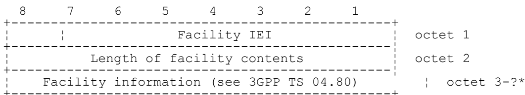
Figure 10.82/3GPP TS 04.08
