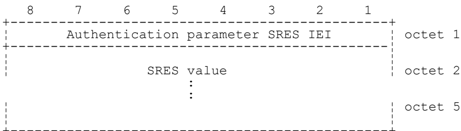
FIGURE 10.62/3GPP TS 04.08 Authentication Parameter SRES information element
