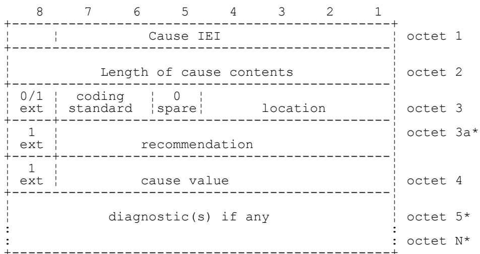
FIGURE 10.77/3GPP TS 04.08 Cause information element
