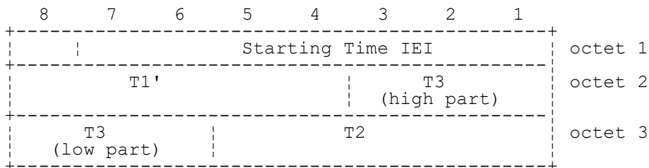
FIGURE 10.55/3GPP TS 04.08 Starting Time information element
