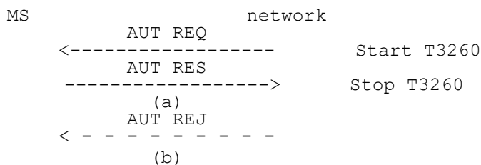
Figure 4.2/3GPP TS 04.08 Authentication sequence: (a) authentication; (b) authentication rejection.
