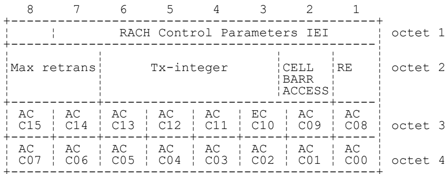
FIGURE 10.47/3GPP TS 04.08 RACH Control Parameters information element
