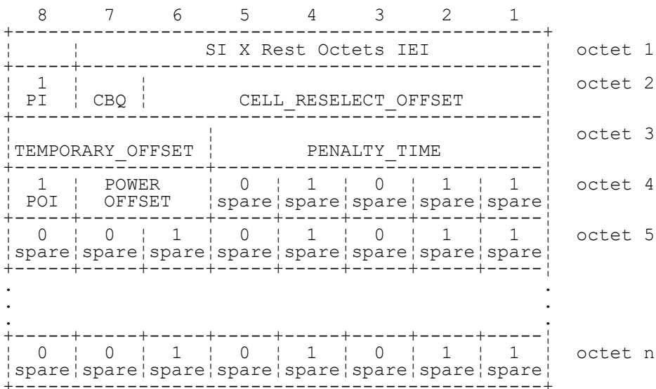
FIGURE 10.53/3GPP TS 04.08 SI X Rest Octets information element (X = 4, 7, or 8), for PI=1 & POI=1
