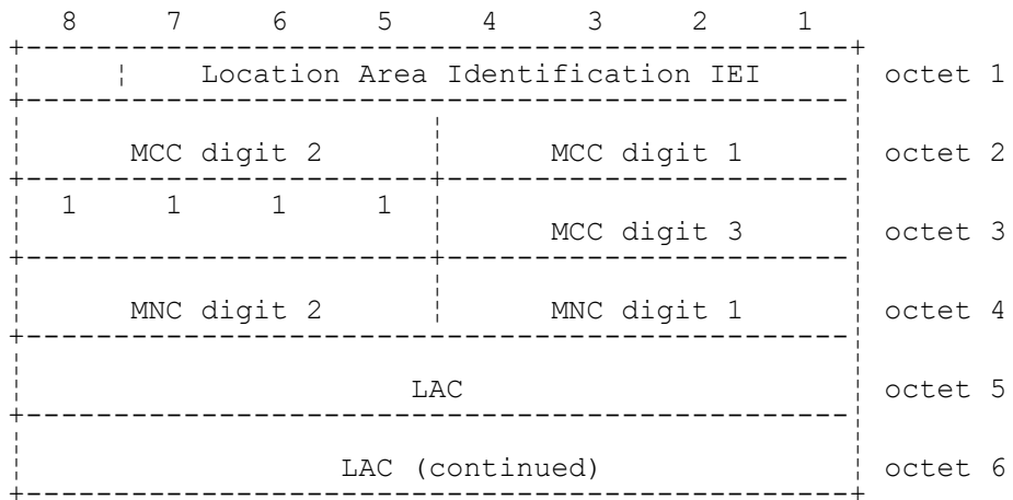
FIGURE 10.4/3GPP TS 04.08 Location Area Identification information element
