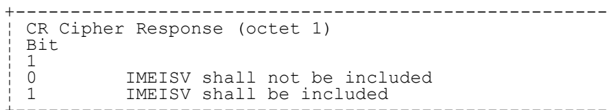
FIGURE 10.24/3GPP TS 04.08 Cipher Response information element
