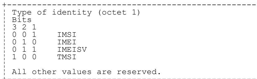
FIGURE 10.64/3GPP TS 04.08 Identity Type information element
