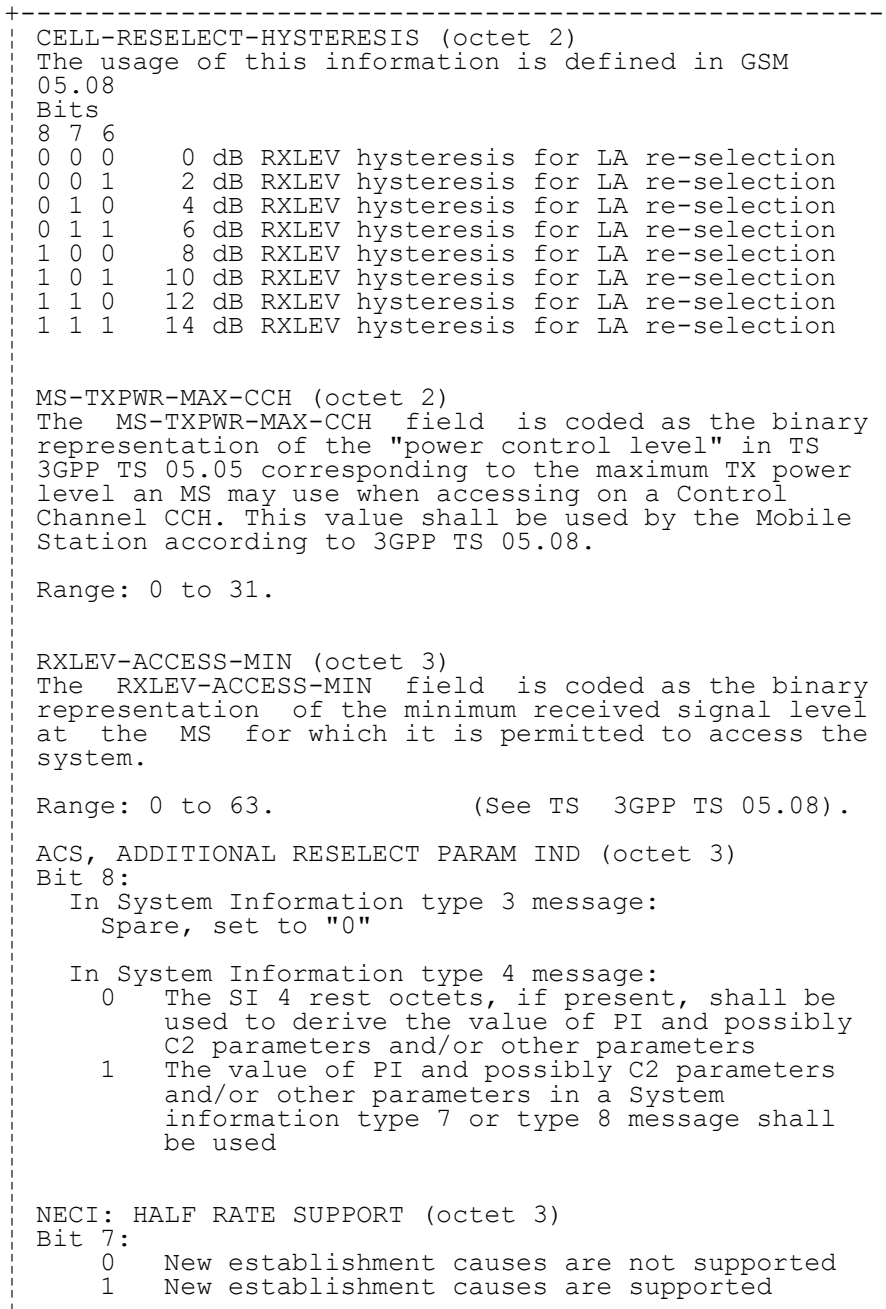
FIGURE 10.18/3GPP TS 04.08 Cell Selection Parameters information element
