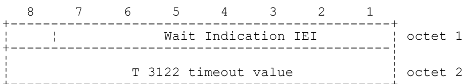
FIGURE 10.60/3GPP TS 04.08 Wait Indication information element
