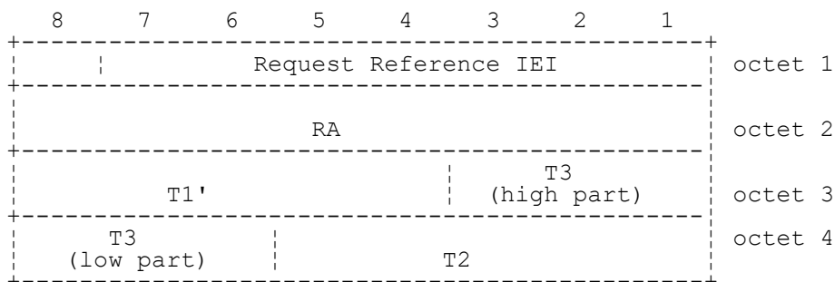
FIGURE 10.48/3GPP TS 04.08 Request Reference information element
