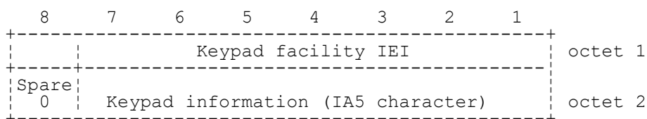
FIGURE 10.84/3GPP TS 04.08 Keypad facility information element
