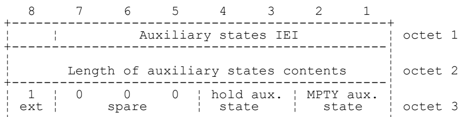
FIGURE 10.70/3GPP TS 04.08 Auxiliary states information element
