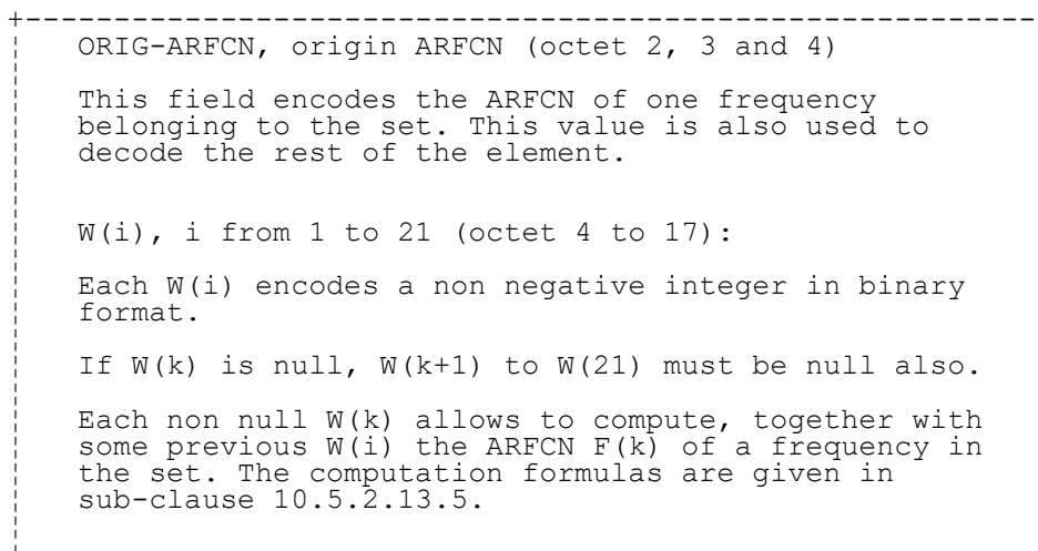
FIGURE 10.13/3GPP TS 04.08 Cell Channel Description information element, range 256 format
