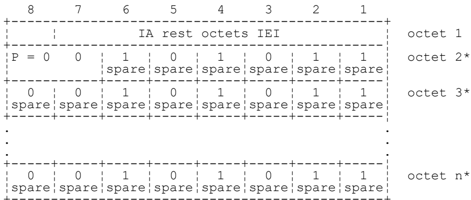
FIGURE 10.34/3GPP TS 04.08 IA rest octets information element, P=00
