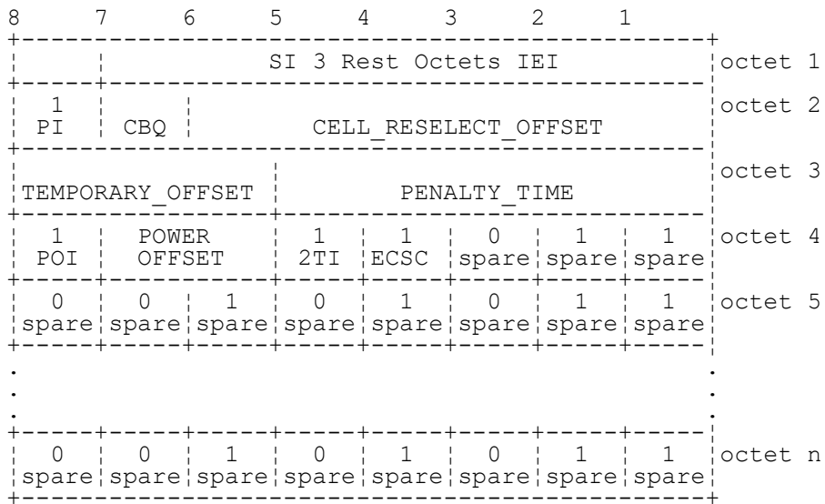
FIGURE 10.52g/3GPP TS 04.08 SI 3 Rest Octets information element for PI=L & POI=L & 2TI=H & ECSC=L
