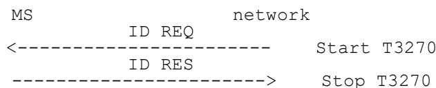
Figure 4.3/3GPP TS 04.08 Identification sequence
