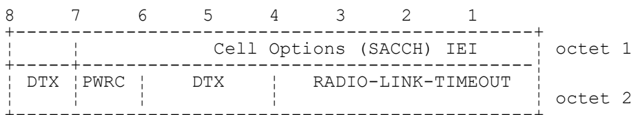
FIGURE 10.17a/3GPP TS 04.08 Cell Options (SACCH) information element
