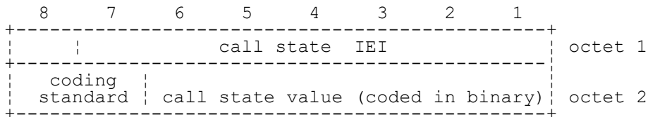
FIGURE 10.72/3GPP TS 04.08 Call state information element
