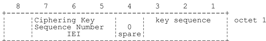
FIGURE 10.3/3GPP TS 04.08 Ciphering Key Sequence Number information element
