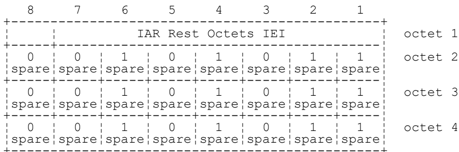
FIGURE 10.35/3GPP TS 04.08 IAR Rest Octets information element
