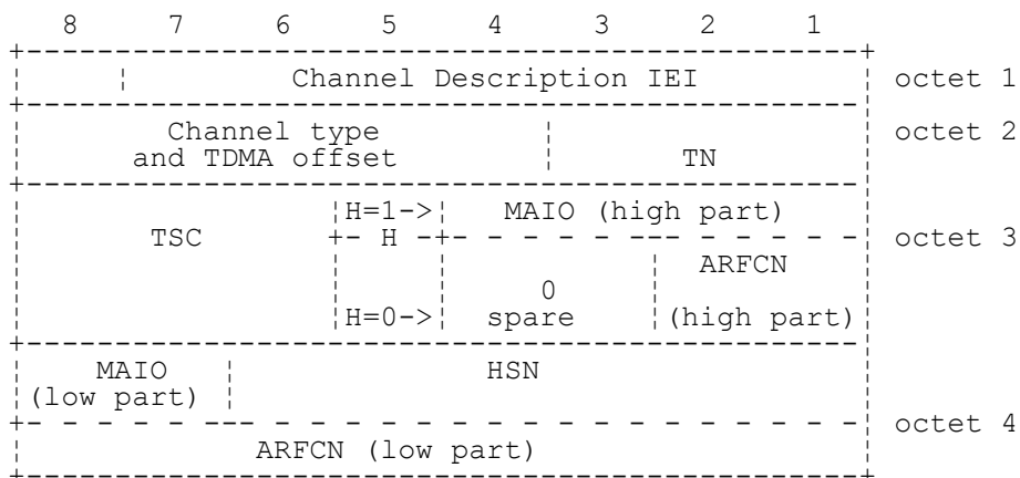
FIGURE 10.19/3GPP TS 04.08 Channel Description information element
