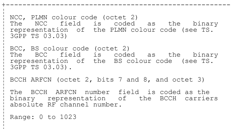
FIGURE 10.16/3GPP TS 04.08 Cell Description information element
