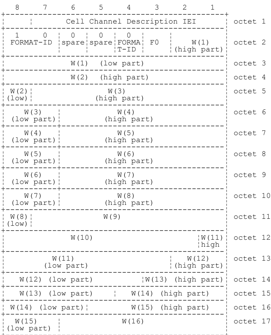
FIGURE 10.11/3GPP TS 04.08 Cell Channel Description information element (1024 range format)
