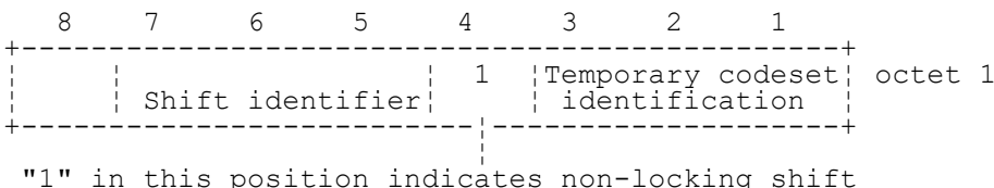
FIGURE 10.69/3GPP TS 04.08 Non-locking shift element
