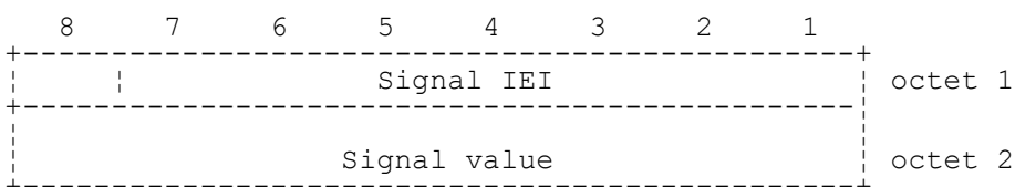
FIGURE 10.90/3GPP TS 04.08 Signal information element
