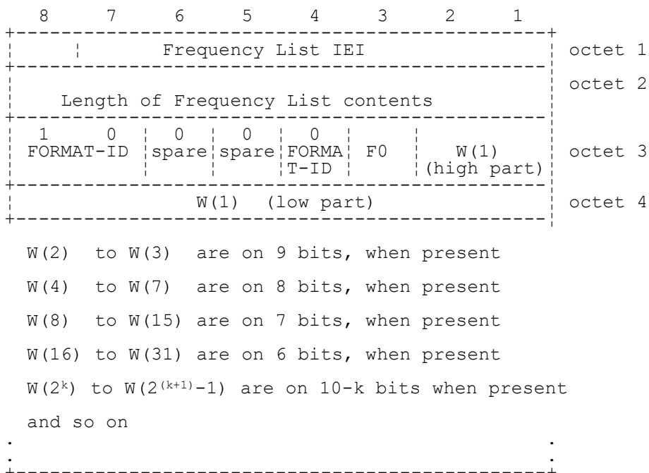
FIGURE 10.28/3GPP TS 04.08 Frequency List information element (Range 1024 format)
