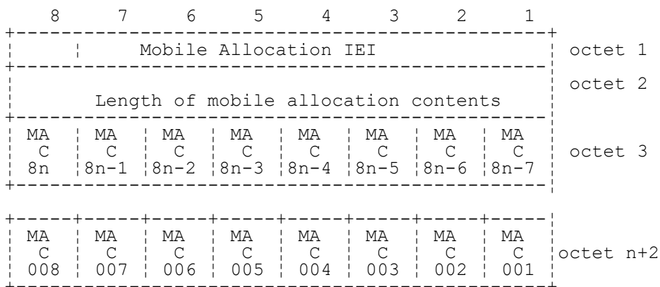
FIGURE 10.39/3GPP TS 04.08 Mobile Allocation information element.
