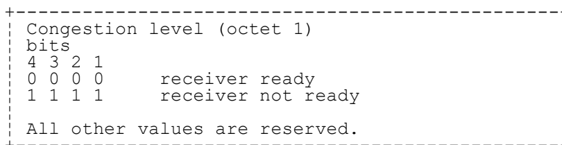
FIGURE 10.79/3GPP TS 04.08 Congestion level information element
