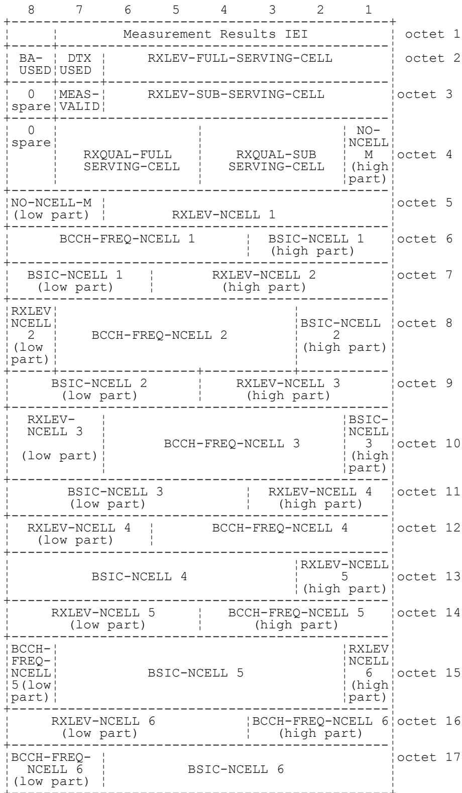
FIGURE 10.38/3GPP TS 04.08 Measurement Results information element
