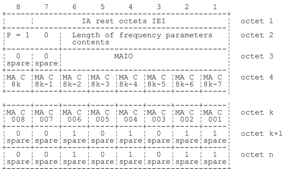
FIGURE 10.34a/3GPP TS 04.08 IA Rest Octets information element, P=10
