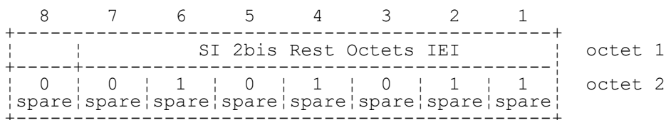
FIGURE 10.51/3GPP TS 04.08 SI 2bis Rest Octets information element
