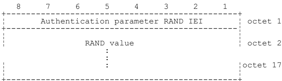
FIGURE 10.61/3GPP TS 04.08 Authentication Parameter RAND information element
