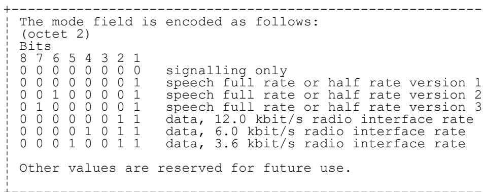
FIGURE 10.20/3GPP TS 04.08 Channel Mode information element
