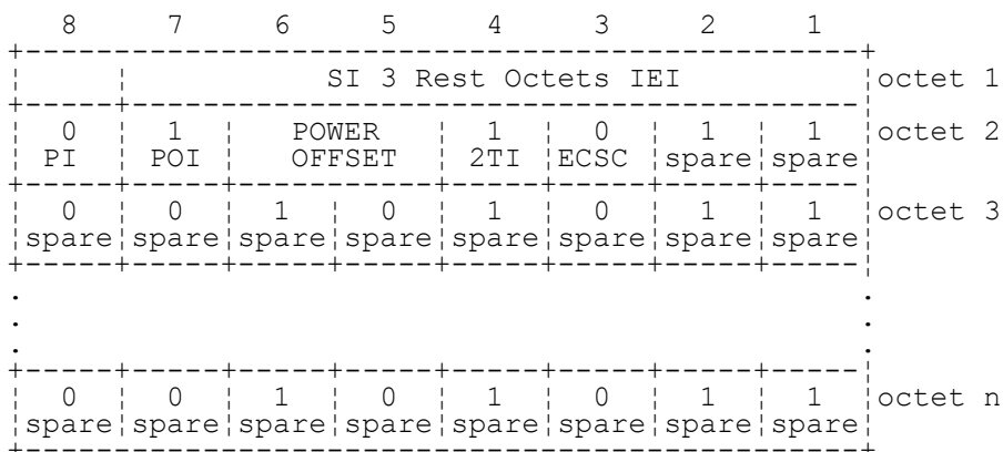
FIGURE 10.52j/3GPP TS 04.08 SI 3 Rest Octets information element for PI=L & POI=H & 2TI=L & ECSC=L
