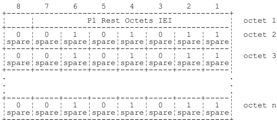
FIGURE 10.41/3GPP TS 04.08 P1 Rest Octets information element
