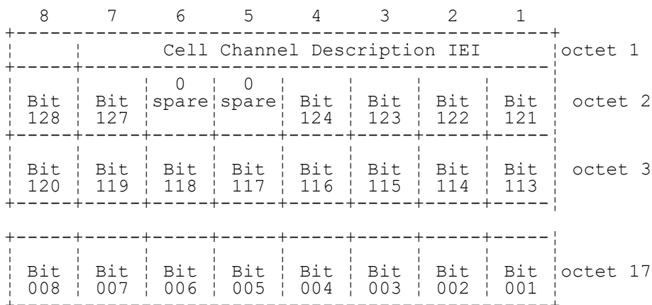
FIGURE 10.9/3GPP TS 04.08 Cell Channel Description information element (general format)
