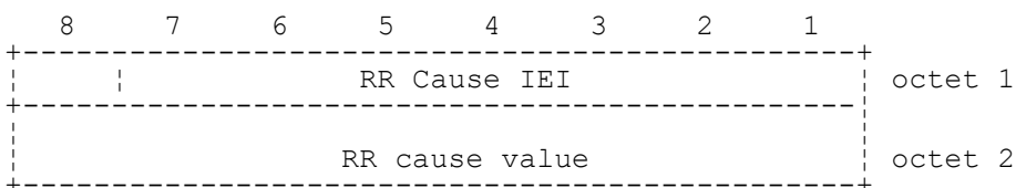
FIGURE 10.49/3GPP TS 04.08 RR Cause information element
