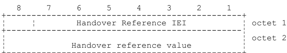
FIGURE 10.33/3GPP TS 04.08 Handover Reference information element
