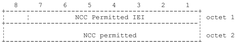
FIGURE 10.45/3GPP TS 04.08 NCC Permitted information element
