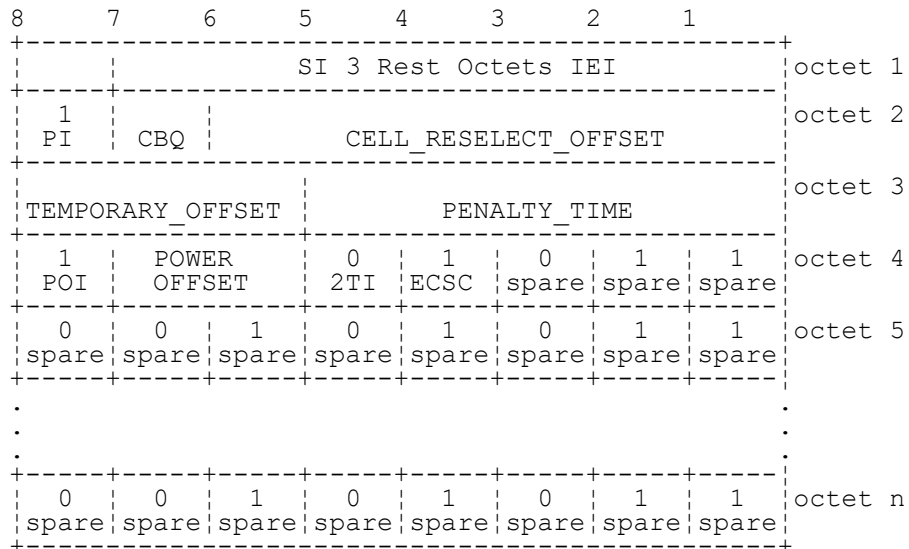
FIGURE 10.52d/3GPP TS 04.08 SI 3 Rest Octets information element for PI=H & POI=H & 2TI=L & ECSC=L
