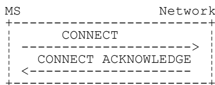
Figure 5.7/3GPP TS 04.08 Call acceptance and active indication at mobile terminating call establishment
