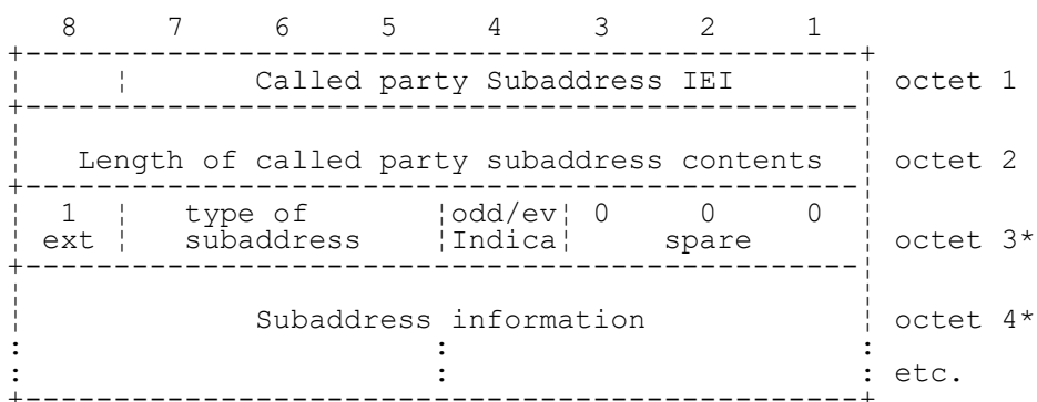
FIGURE 10.74/3GPP TS 04.08 Called party subaddress
