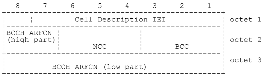
FIGURE 10.16/3GPP TS 04.08 Cell Description information element
