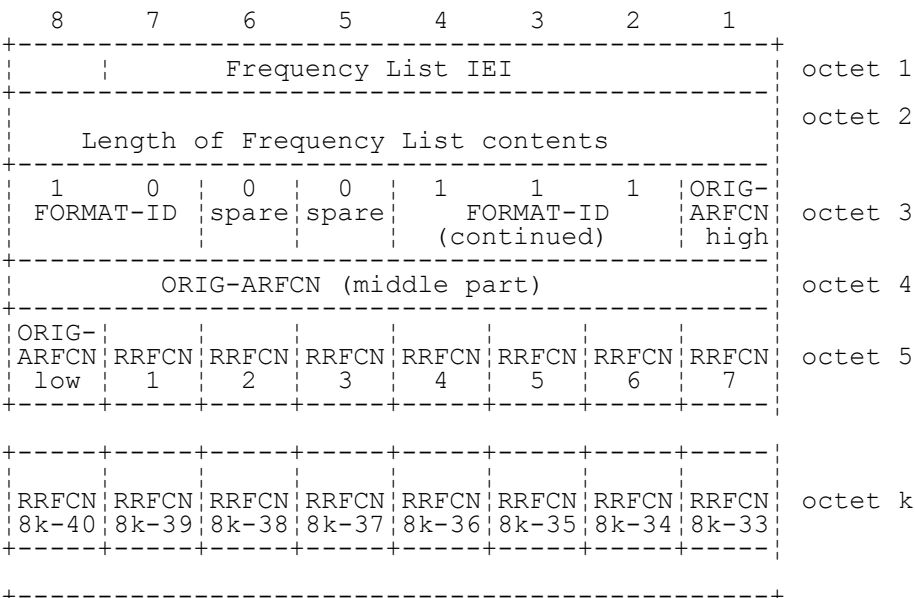
FIGURE 10.32/3GPP TS 04.08 Frequency List information element, variable bit map format
