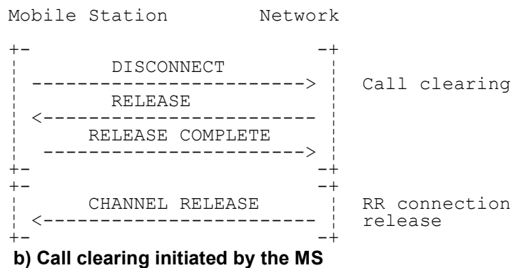
Figure 7.12/3GPP TS 04.08 Call clearing
