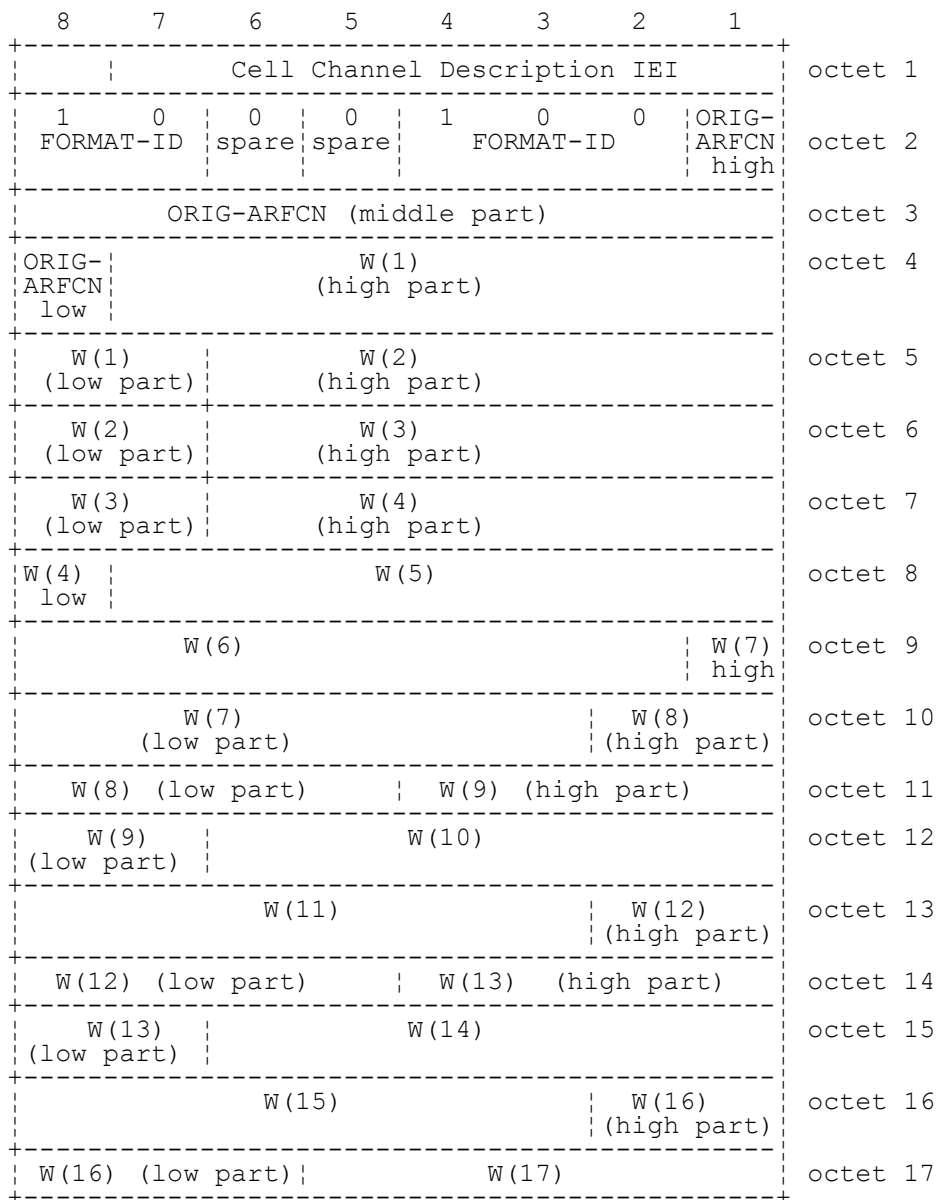
FIGURE 10.12/3GPP TS 04.08 Cell Channel Description information element (512 range format)
