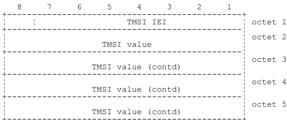
FIGURE 10.59/3GPP TS 04.08 TMSI information element
