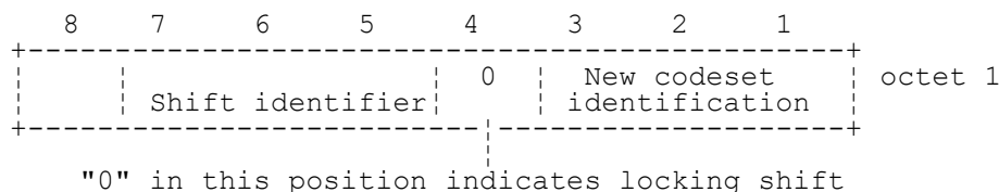
FIGURE 10.68/3GPP TS 04.08 Locking shift element
