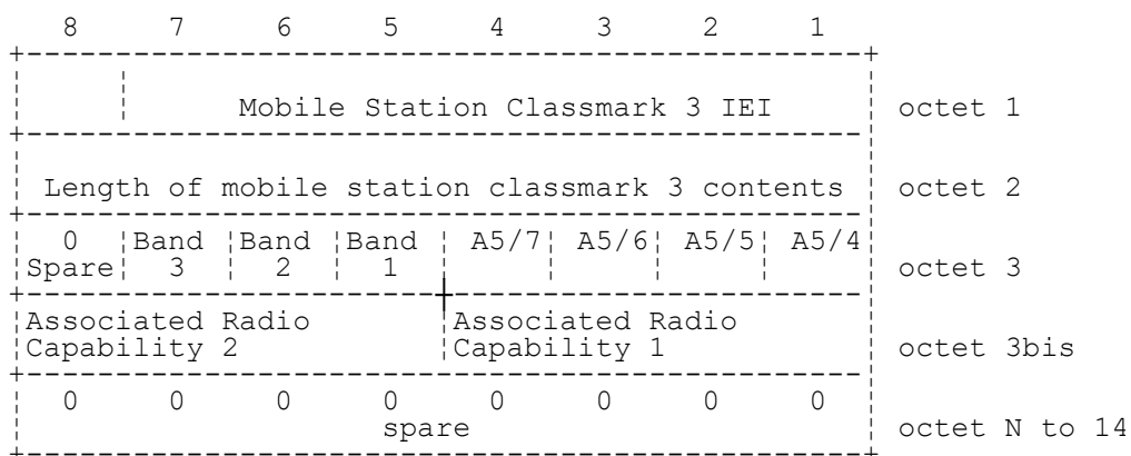
FIGURE 10.8/3GPP TS 04.08 Mobile Station Classmark 3 information element
