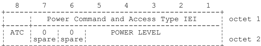
FIGURE 10.46a/3GPP TS 04.08 Power Command and access type information element
