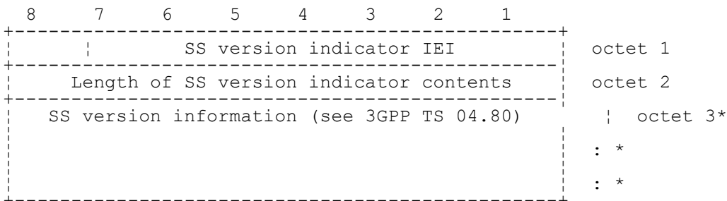
Figure 10.91/3GPP TS 04.08
