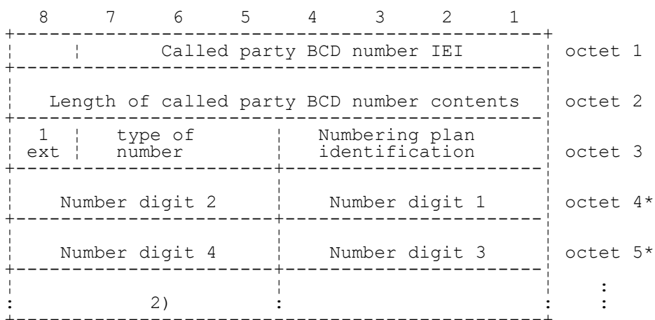
FIGURE 10.73/3GPP TS 04.08 Called party BCD number information element
