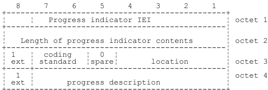
FIGURE 10.88/3GPP TS 04.08 Progress indicator information element
