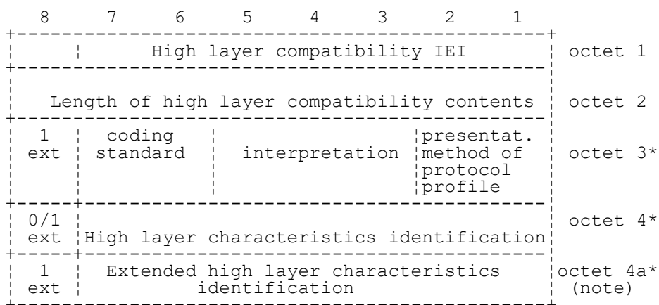
FIGURE 10.83/3GPP TS 04.08 High layer compatibility information element
