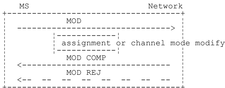
Figure 5.10a/3GPP TS 04.08 In-call modification sequence initiated by MS
