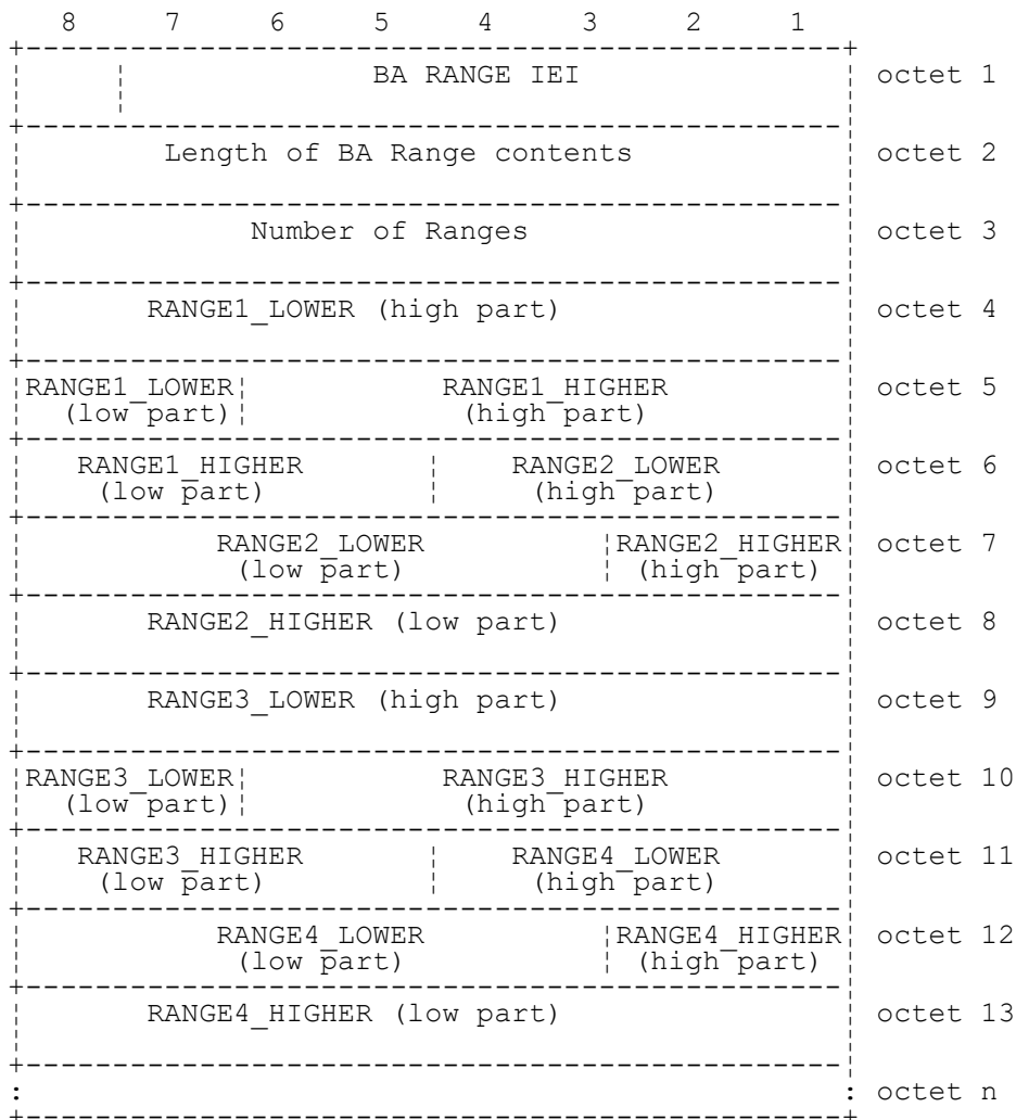
FIGURE 10.8a/3GPP TS 04.08 BA RANGE information element
