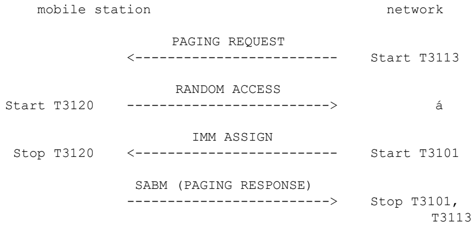
Figure 3.2/3GPP TS 04.08 Paging sequence
