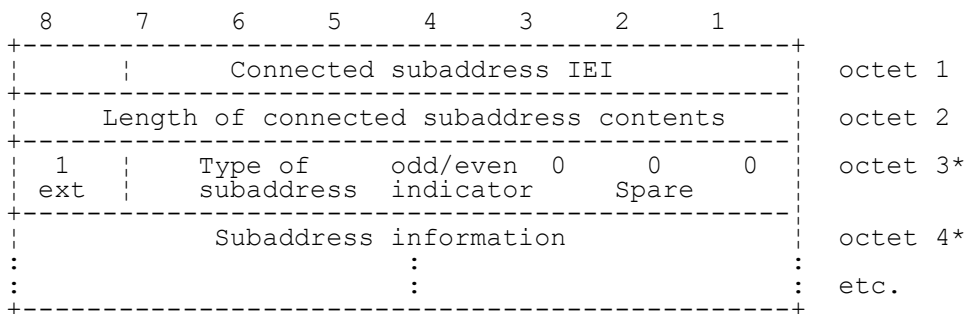
Figure 10.81/3GPP TS 04.08
