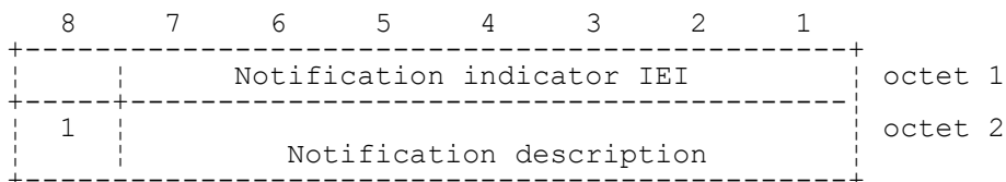
FIGURE 10.87/3GPP TS 04.08 Notification indicator information element
