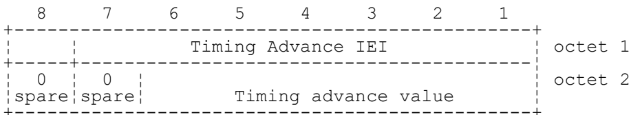
FIGURE 10.57/3GPP TS 04.08 Timing Advance information element
