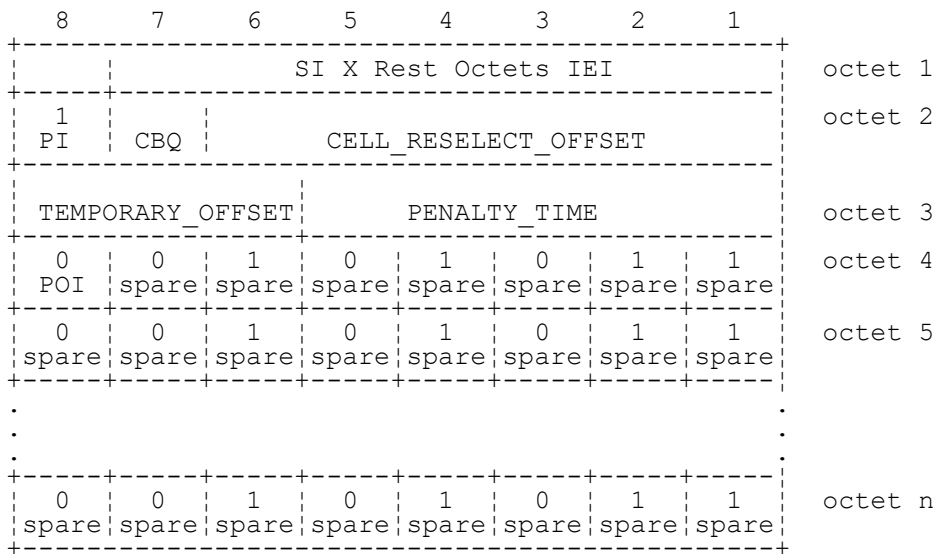
FIGURE 10.54a/3GPP TS 04.08 SI X Rest Octets information element (X = 4, 7, or 8), for PI=1 & POI=0
