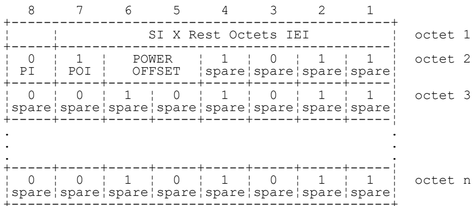
FIGURE 10.54b/3GPP TS 04.08 SI X Rest Octets information element (X = 4, 7, or 8), for PI=0 & POI=1
