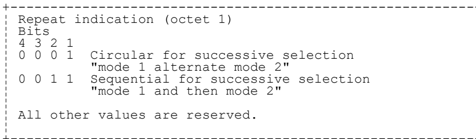
FIGURE 10.89/3GPP TS 04.08 Repeat indicator information element
