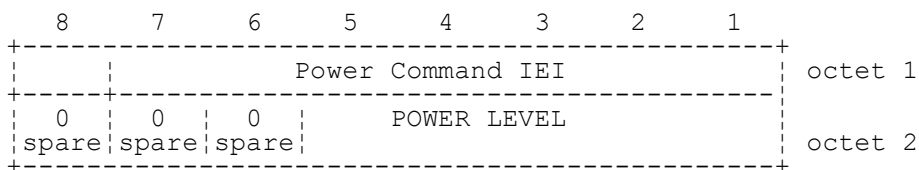
FIGURE 10.46/3GPP TS 04.08 Power Command information element
