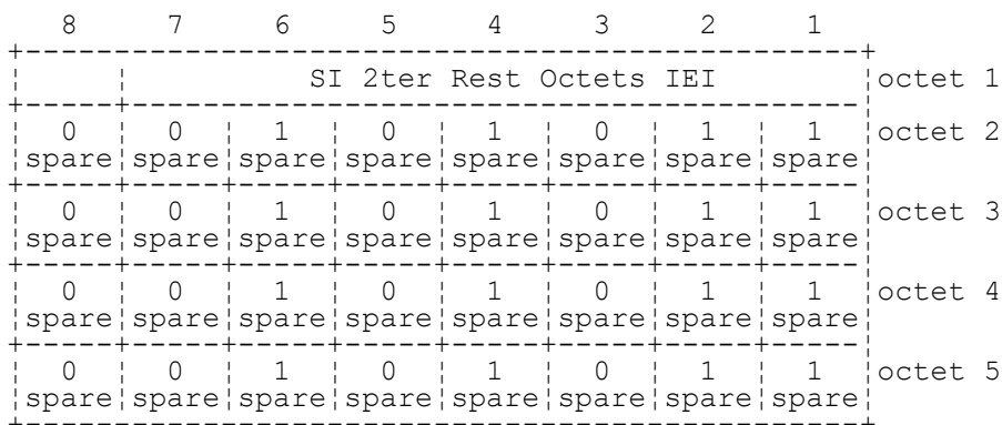
FIGURE 10.51a/3GPP TS 04.08 SI 2ter Rest Octets information element
