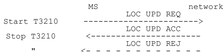
Figure 4.5/3GPP TS 04.08 Location updating sequence
