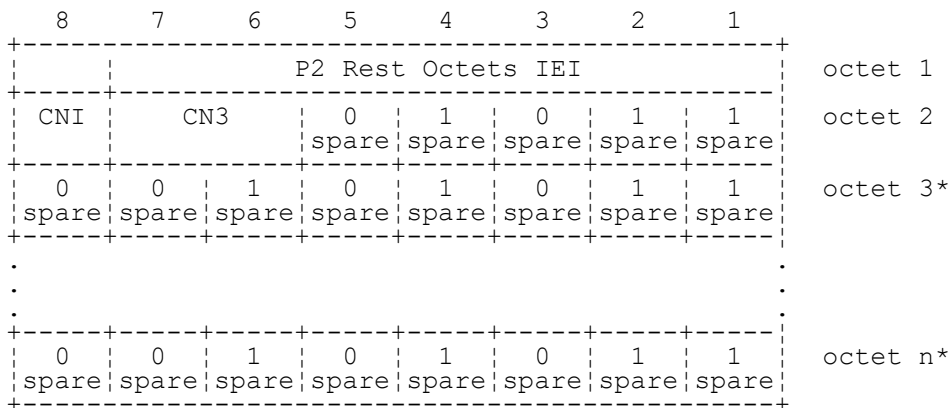
FIGURE 10.42/3GPP TS 04.08 P2 Rest Octets information element
