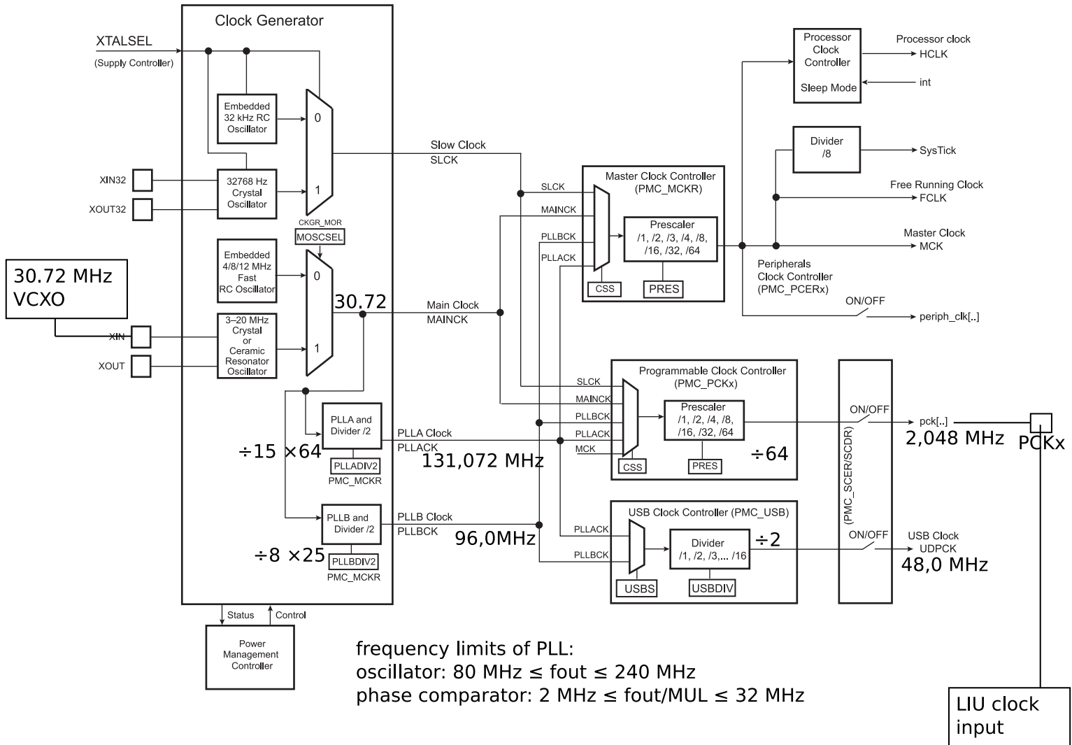
Figure 29-1. General Clock Block Diagram
