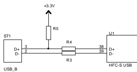
Figure 17: USB connection
