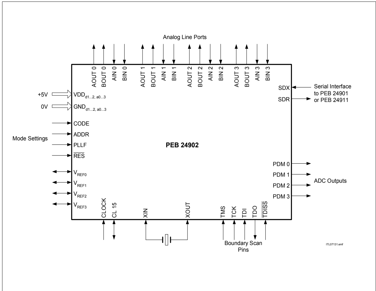
Figure 1 Logic Symbol
